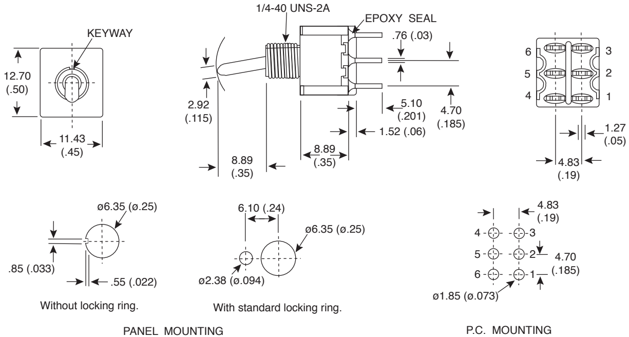
PANEL MOUNTING
